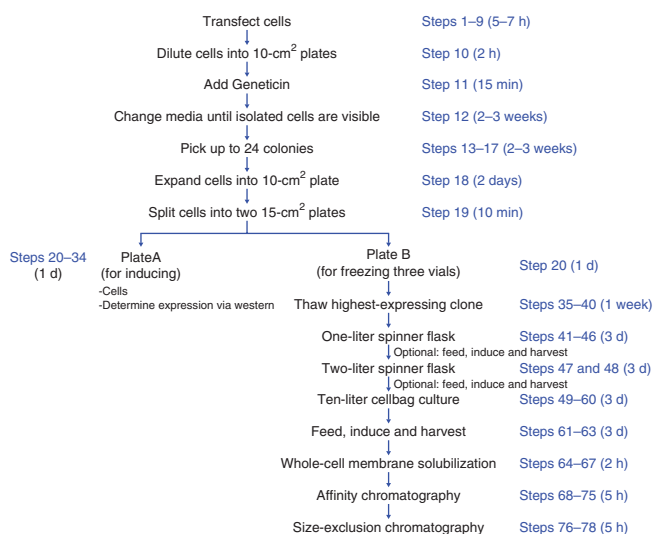
Figure 2 | Workflow for the overexpression of mammalian membrane proteins in stably transfected and clonal HEK293S GnTI - cells.
