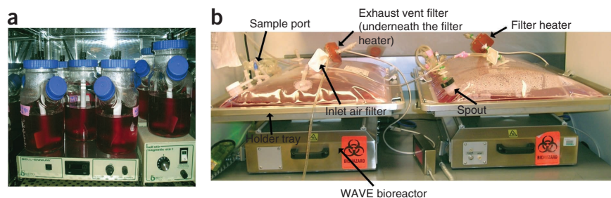
Figure 5 | Medium- and large-scale HEK293S GnTI - cell cultures. (a) Up to seven 1-liter spinner flasks can be maintained in a single CO 2 incubator. Alternatively, up to three 3-liter spinner flasks can be maintained (not shown). (b) Two 10-liter WAVE bioreactors, using cellbags manufactured by GE Healthcare (left) and Flex Concepts Inc. (right), are shown. Relevant features of the cellbag and WAVE bioreactor, as discussed in the text, are highlighted.
