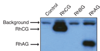
Figure 1 | Expression testing of full-length human Rh membrane proteins in transiently transfected HEK293S GnTI - cells. A measure of 10 µg of RhAG, RhBG and RhCG, subcloned into pACMV-tetO, was separately transfected into HEK293S GnTI - cells grown in a 10-cm 2 tissue culture plate. Cells were induced with doxycycline (24 h after transfection), collected (24 h post induction) and analyzed via anti-histidine western blotting, as described in the text. On the basis of these results, RhAG and RhCG were chosen as candidates for stable cell line generation.
